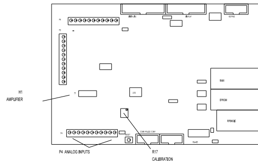
Figure 10-1 Analog I/O
